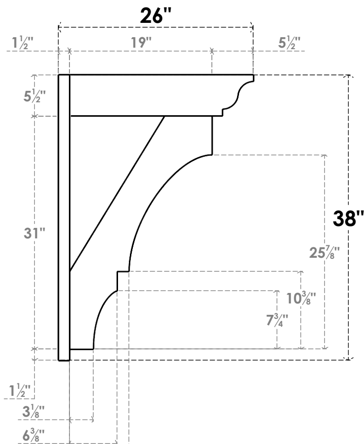
SIDE PROFILE
