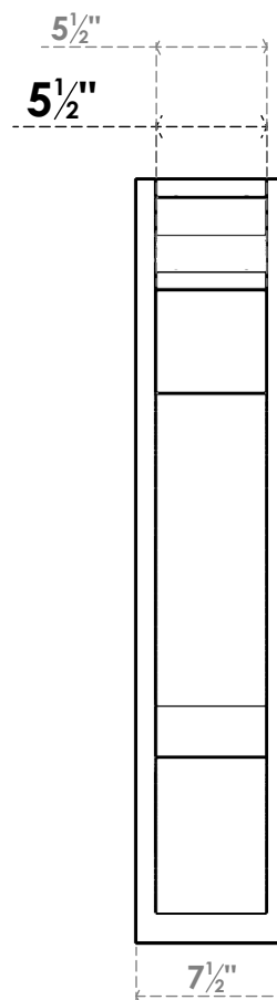
FRONT PROFILE
